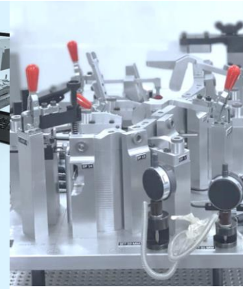
Checking Fixtures & Smart gauges
